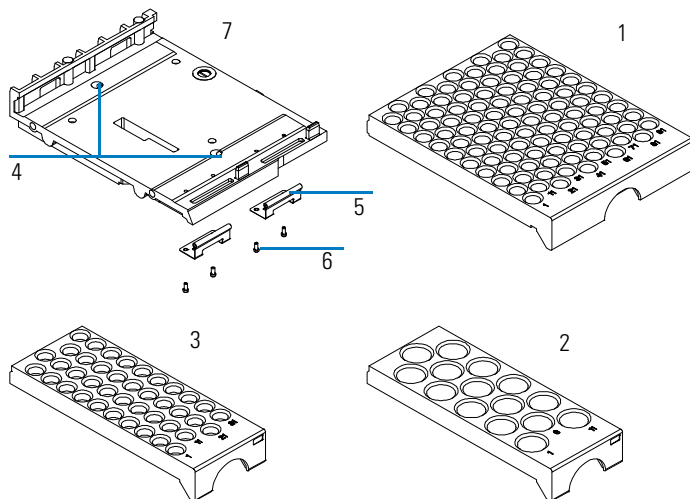
Vial Trays and Tray Base
